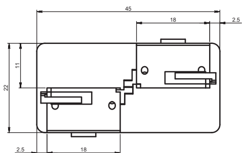
PA-1_0.43_100W
